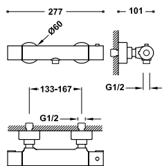
Wall-mounted thermostatic shower mixer tap Anti-limescale: Ø 100 mm hand shower. Adjustable support for hand shower. Metal hose.
