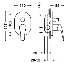
2-way concealed single-handle shower mixer tap Concealed body included. 2-way diverter.
