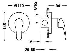
1-way concealed single-handle shower mixer tap Concealed body included.
