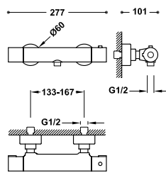
Wall-mounted thermostatic shower mixer tap Without accessories.
