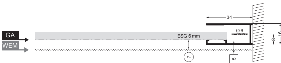
SLIDE side screen next to triple sliding door
