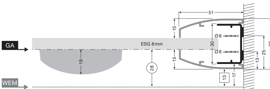
ARTWEGER 360 Walk In partially framed
