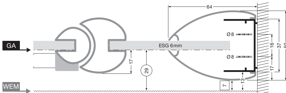
TWISTLINE with fixed part
