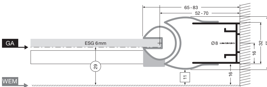
ARTWEGER 360 partially framed without fixed part
