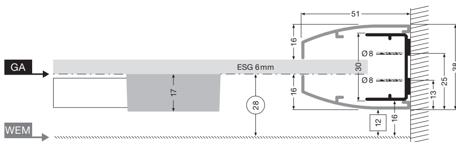
ARTWEGER 360 partially framed with fixed part
