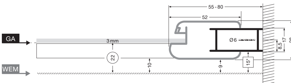
BASELINE *side screen 10mm
