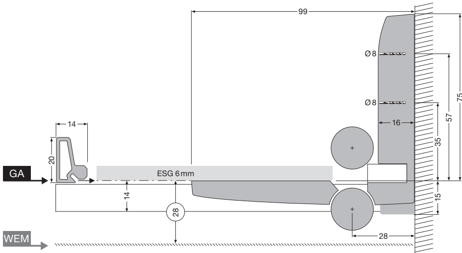
ARTWEGER 360 frameless without fixed part
