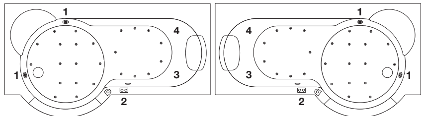
TWINLINE 1 AIR arrangement of equipment
