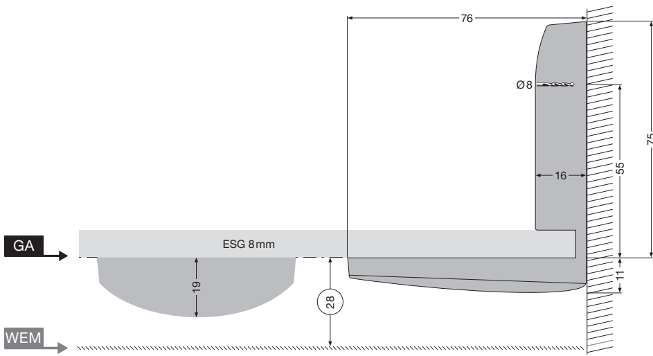
ARTWEGER 360 Walk In frameless Brackets inwards
