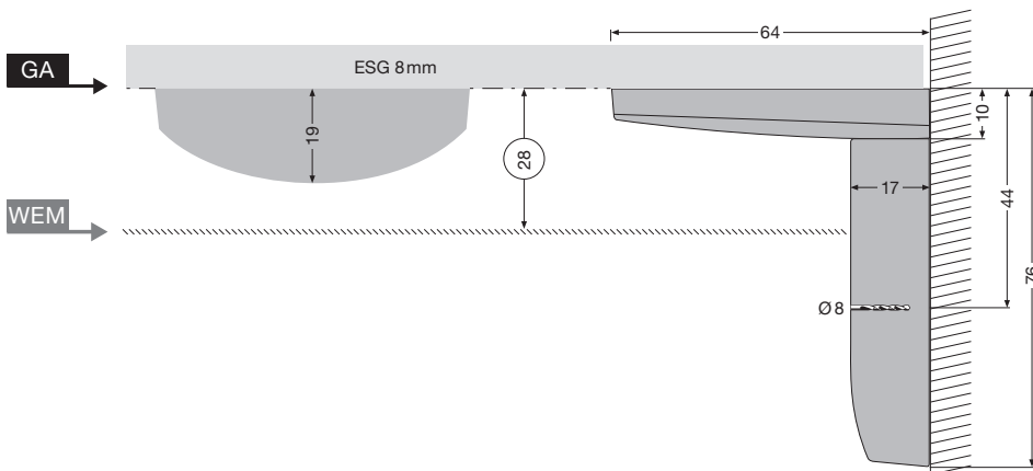
ARTWEGER 360 Walk In frameless Brackets outwards
