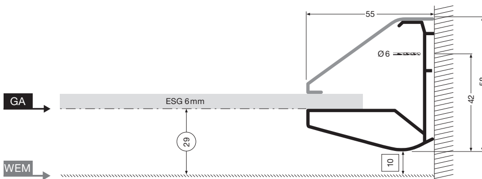
LIFELINE side screen
