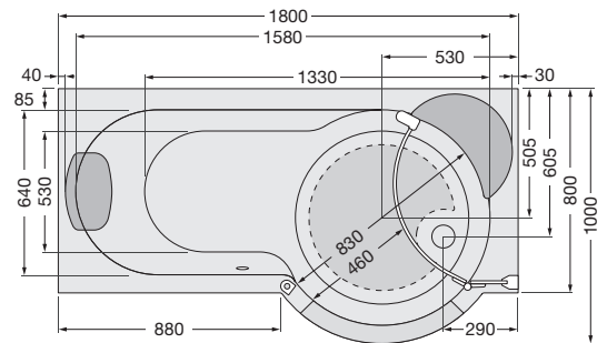
TWINLINE 1 1800 x 1000 / 800 depth 430
